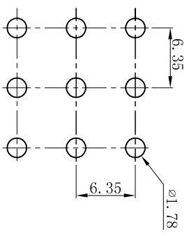
P.C.B LAYOUT: TOP VIEW TOLERANCE: ±0.05mm
