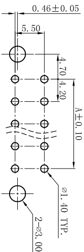
P.C.B LAYOUT: TOP VIEW TOLERANCE: ± 0.05mm
