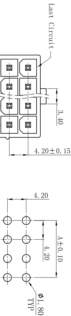
P.C.B LAYOUT: TOP VIEW TOLERANCE: ±0.05mm
