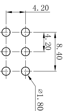
P.C.B LAYOUT: TOP VIEW TOLERANCE: ±0.05mm
