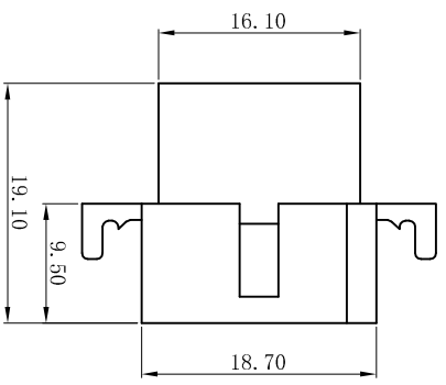
H3682-04P H3682NE-04P
