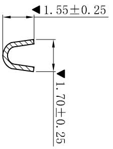
SECTION: C-C
