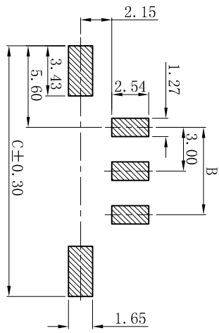
P.C.B Layout: TOP VIEW Tolerance: ±0.05mm
