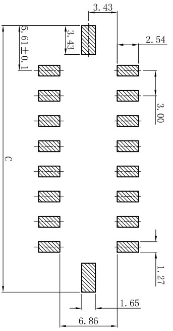
P.C.B Layout: TOP VIEW Tolerance: ±0.05mm
