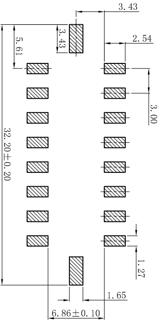
P.C.B Layout: TOP VIEW Tolerance: ±0.05mm
