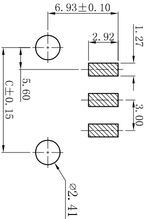
P.C.B Layout: TOP VIEW Tolerance: ±0.05mm
