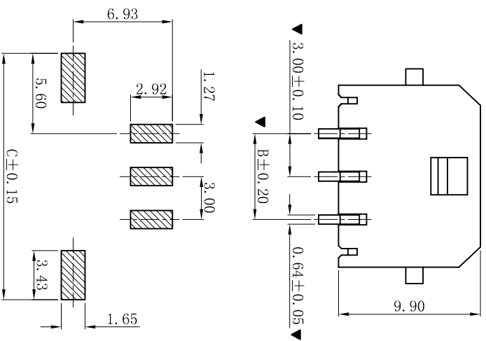
P.C.B Layout: TOP VIEW Tolerance: ±0.05mm
