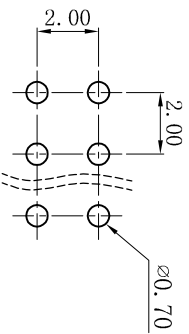
P. C. B LAYOUT
