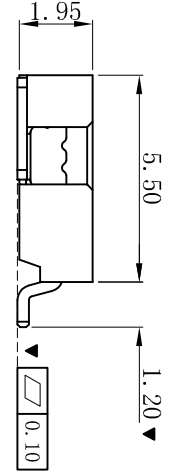
02P~03P Single Hole Scale 1:1
