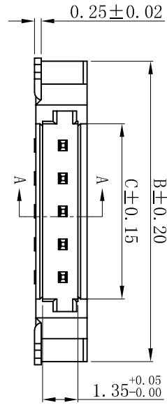
04P~30P Double Hole Scale 1:1
