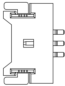
02P~03P Single Hole Scale 1:1
