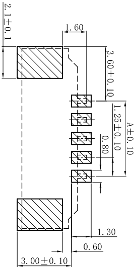
P.C.B LAYOUT: TOP VIEW TOLERANCE: ±0.05mm
