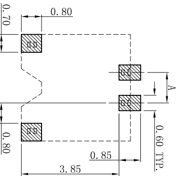
P.C.B LAYOUT: TOP VIEW TOLERANCE: ±0.05mm
