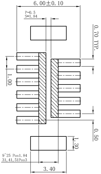
P.C.B LAYOUT: TOP VIEW TOLERANCE: ±0.05mm
