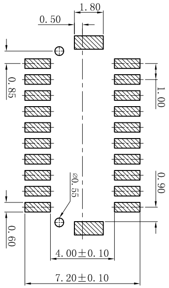
P.C.B LAYOUT: TOP VIEW TOLERANCE: ±0.05mm
