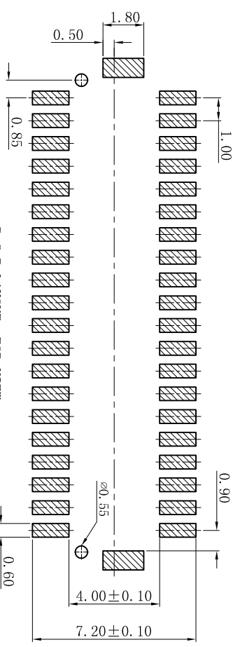
P.C.B LAYOUT: TOP VIEW TOLERANCE: ±0.05mm
