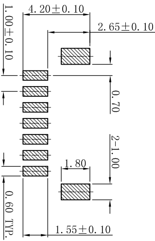
P.C.B LAYOUT: TOP VIEW TOLERANCE: ±0.05mm
