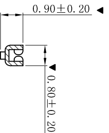
SEC C-C
